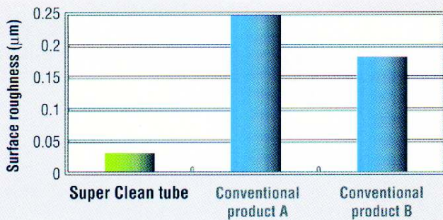
Fig. 1 Measurement result of surface roughness (Ra)
