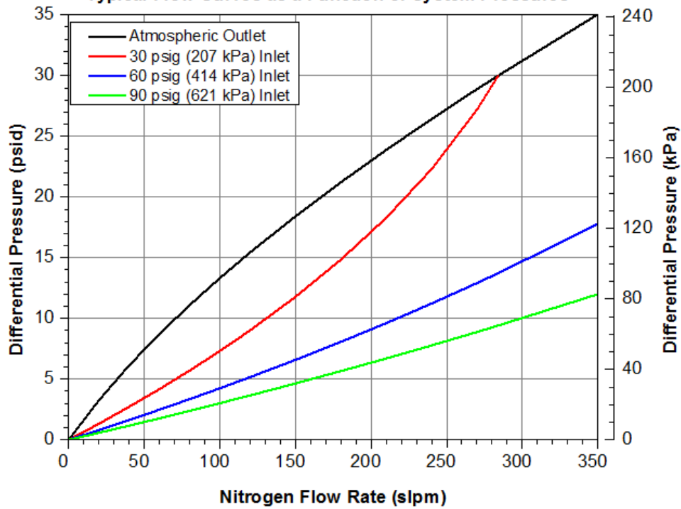
Mott DEF315H Flow Rate vs. Differential Pressure Typical Flow Curves as a Function of System Pressures
