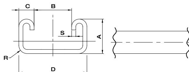
BLANK STAINLESS STEEL TUBE HOLDER SUPPORT
