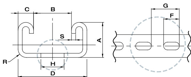
PERFORATED STAINLESS STEEL TUBE HOLDER SUPPORT
