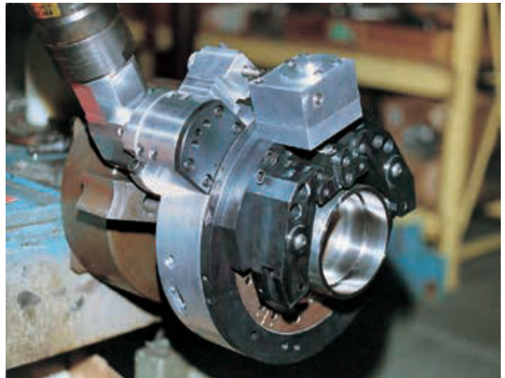
A small SB lathe fitted with a cut-off wheel module performs "chipless" cutting of thin-wall tubing.
