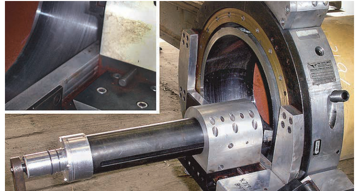
Clamshell configured to perform extremely accurate deep counterboring.
