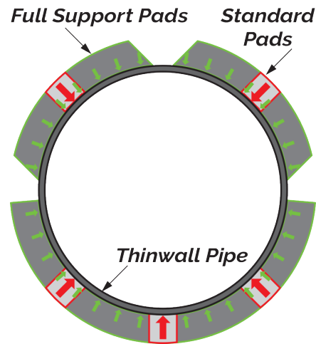
An illustration showing distribution of clamping force, a comparison is easy to make between the standard (Red) and Full Support Pads (Green).
