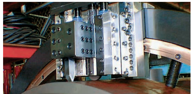
An OD Tracking Module accessory being utilized on a large SB clamshell. The Tracking Module compensates for out-of-round conditions by "reading" the pipe shape with a wheel, automatically adjusting cut depth.
