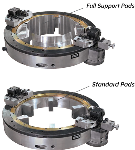
In the 612SB Clamshell shown above, the increased surface area of Full Support Pads is clearly seen. While conventional Clamshell mounting pads provide secure grip on regular to heavy wall pipe, they can focus strong clamping forces that could distort and deform thinner wall thicknesses.
