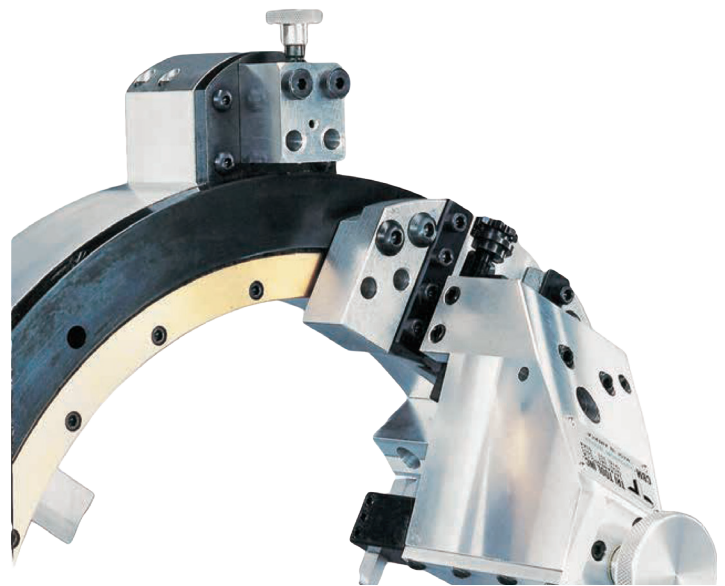
Model CBM-2 Counterbore Module
