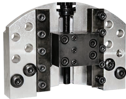
The 3 Position Tool Holder mounting bolts (shown) can be mounted in one of the three positions to shift the module in or out to accommodate different pipe sizes.
