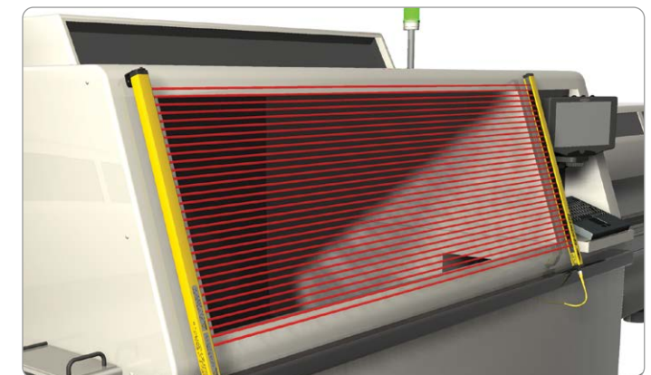
The Type 2 EZ-SCREEN safety light screen guards the opening to a chip shooter, which has moving parts that can cause painful but usually temporary injuries.
